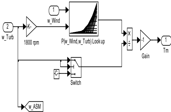
Fig 4 Wind Turbine Model
