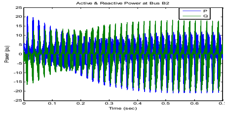
Figure 7 Active Power & Reactive Power at Bus 2
