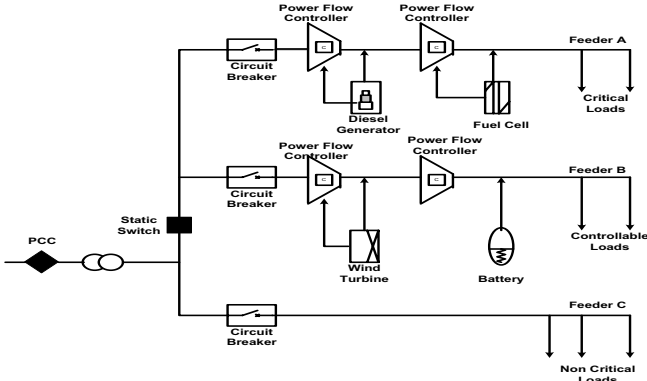
Fig 1 Schematic Microgrid Architecture
