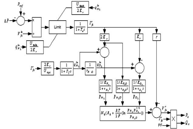
Fig 3 SOFC system dynamic model
