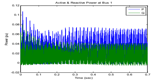
Figure 5 Active Power & Reactive Power at Bus 1
