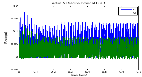
Figure 6 Active Power & Reactive Power at Bus 1
