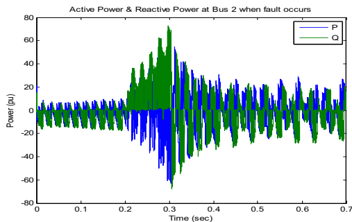
Figure 9 Active & Reactive Power at Bus 2
