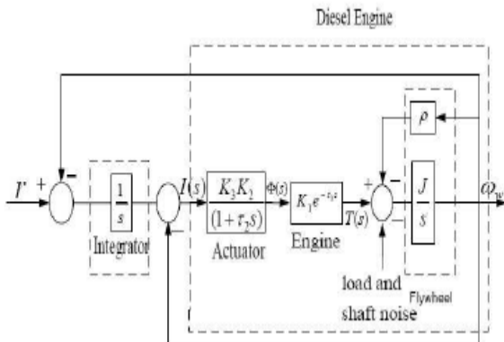
Fig 2 Block Diagram of Diesel Engine system
