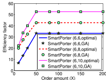
Fig. 2. Validation of the proposed genetic algorithm (GA) compared to the optimal solution. Within first braces the first and second indexes are T_{\min} and T_{\max} respectively.
