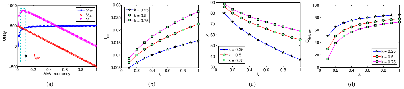
Fig. 8. Variation of (a) different utility functions with AEV frequency. Effect of different package arrival rate \lambda on (b) optimal AEV frequency f_{opt} , (c) percentage of empty miles \mathcal{E} , and (d) the package delivery quality \mathcal{Q}_{delivery} .
