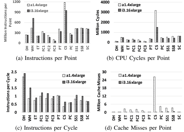
Fig. 2: Cost analysis of the single-thread UnixBench test results on a1.4xlarge and i3.16xlarge instances running on dedicated hosts.
